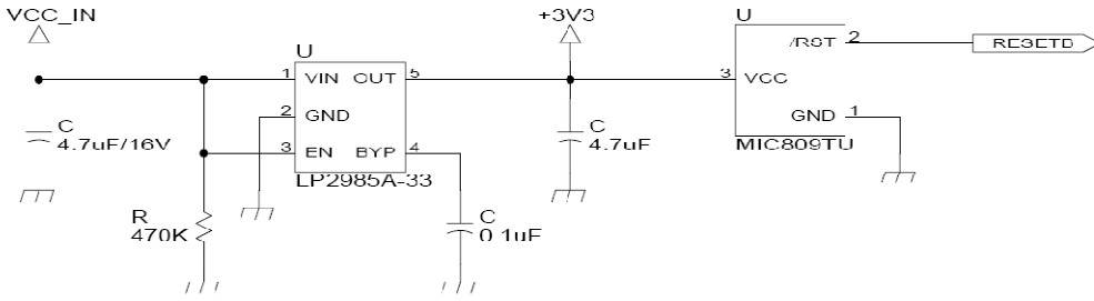
[Power Supply Interface]
