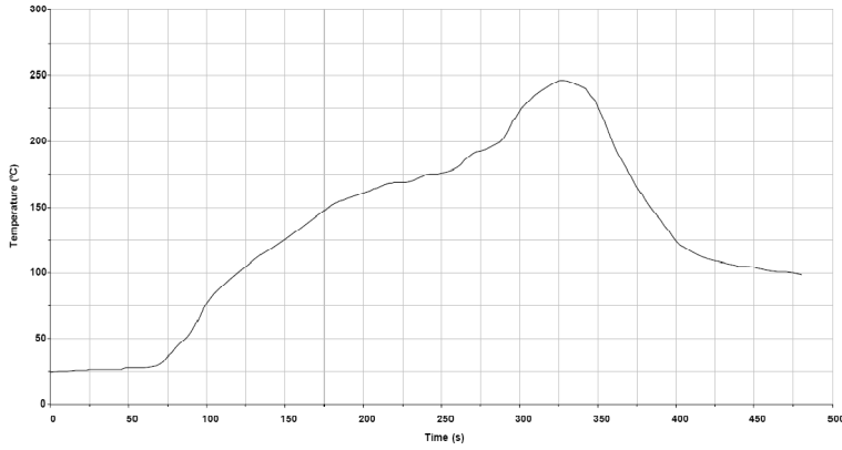
[Typical Lead-Free Re-flow Solder Profile]
