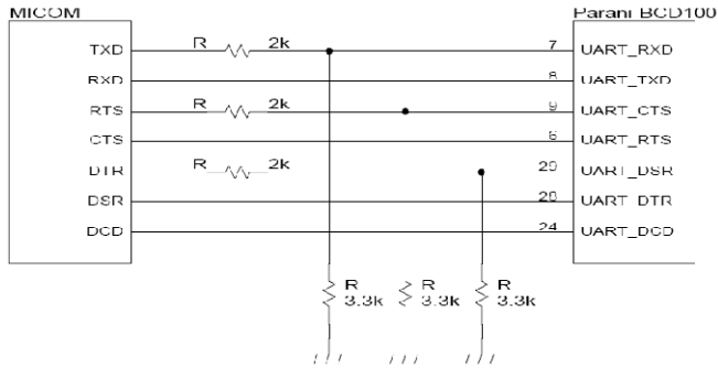
[MICOM UART Interface]
